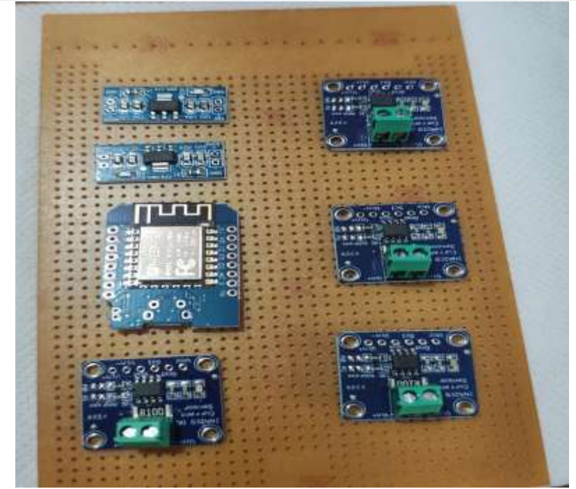
Components Mounted
